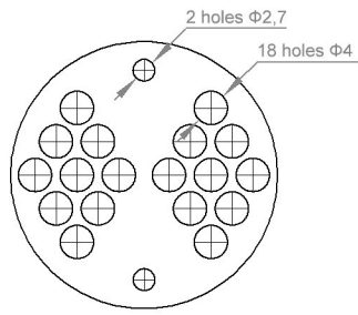
Valve marking template
